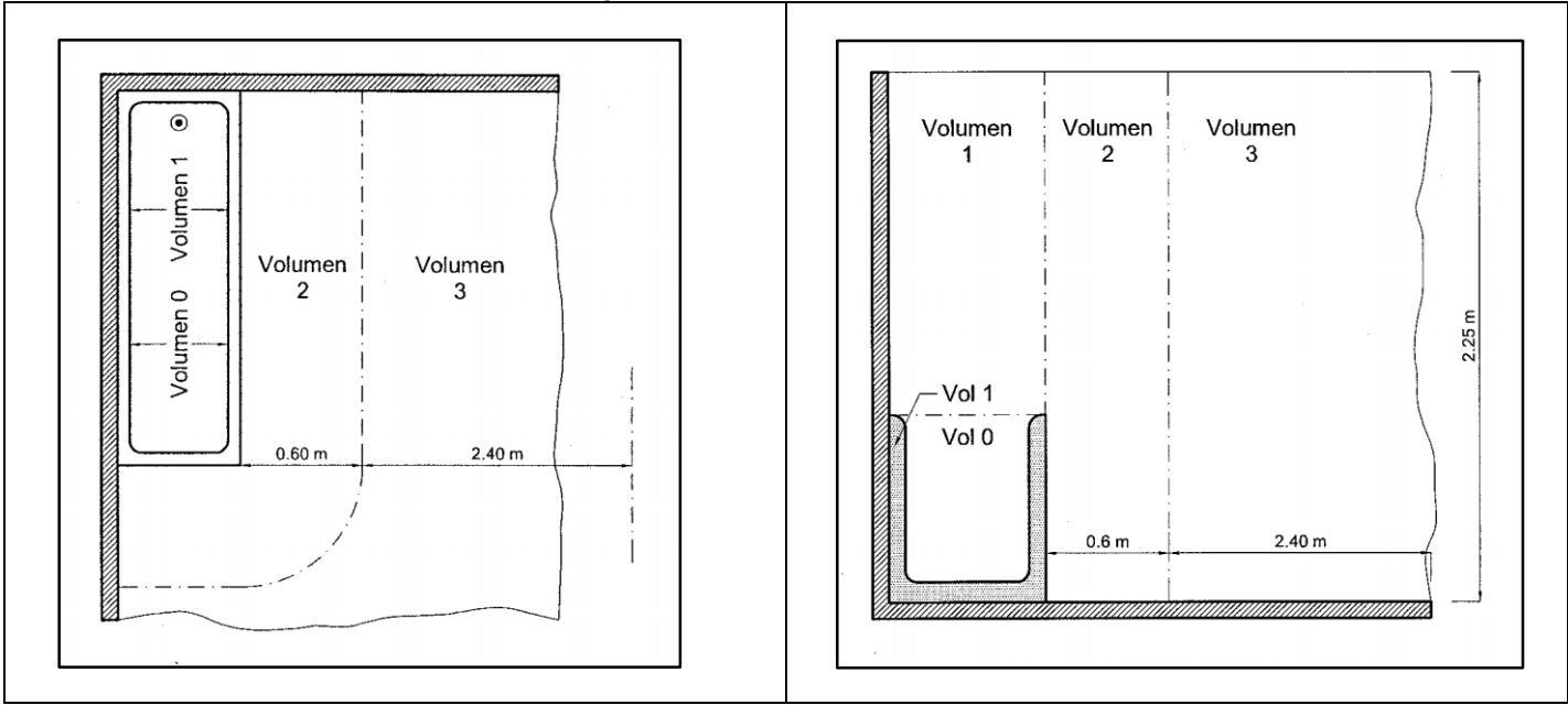
Figura 11.6.1 – BAÑERA
